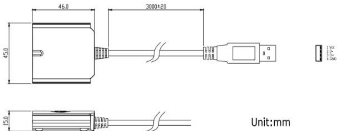
Figure 3: SKM55U-GPS Series Connector
