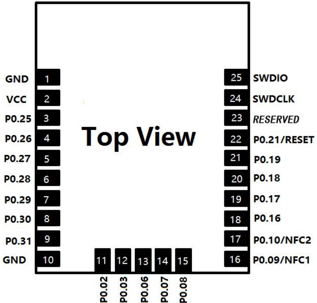
Figure 4: SKB369-AAXXPI Module Pinout
