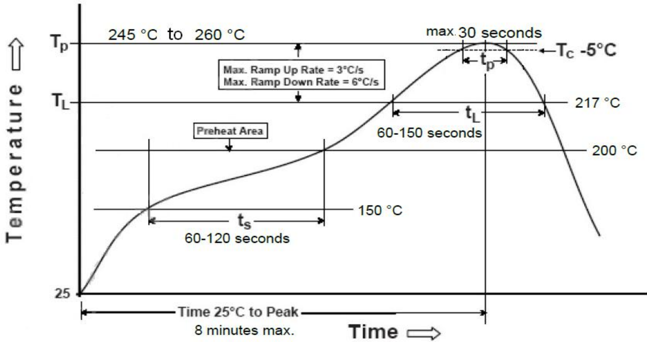
Figure 6: SKB369-AAXXPI Typical Lead-free Soldering Profile
