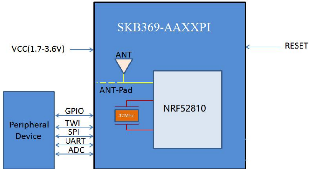
Figure 3: SKB369-AAXXPI Block Diagram
