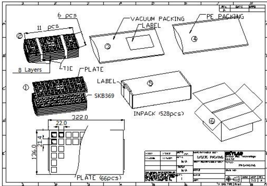
Figure 7: SKB369-AAXXPI Packaging
