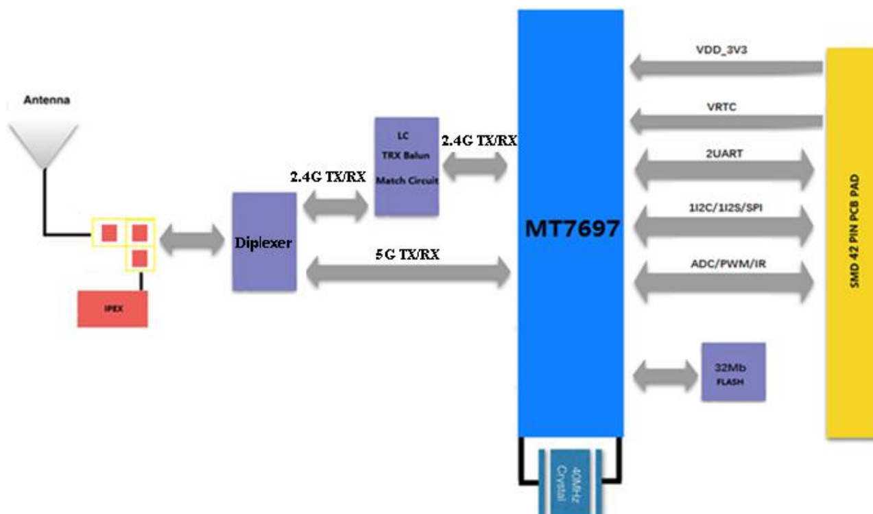
Figure 2: WG222 Block Diagram
