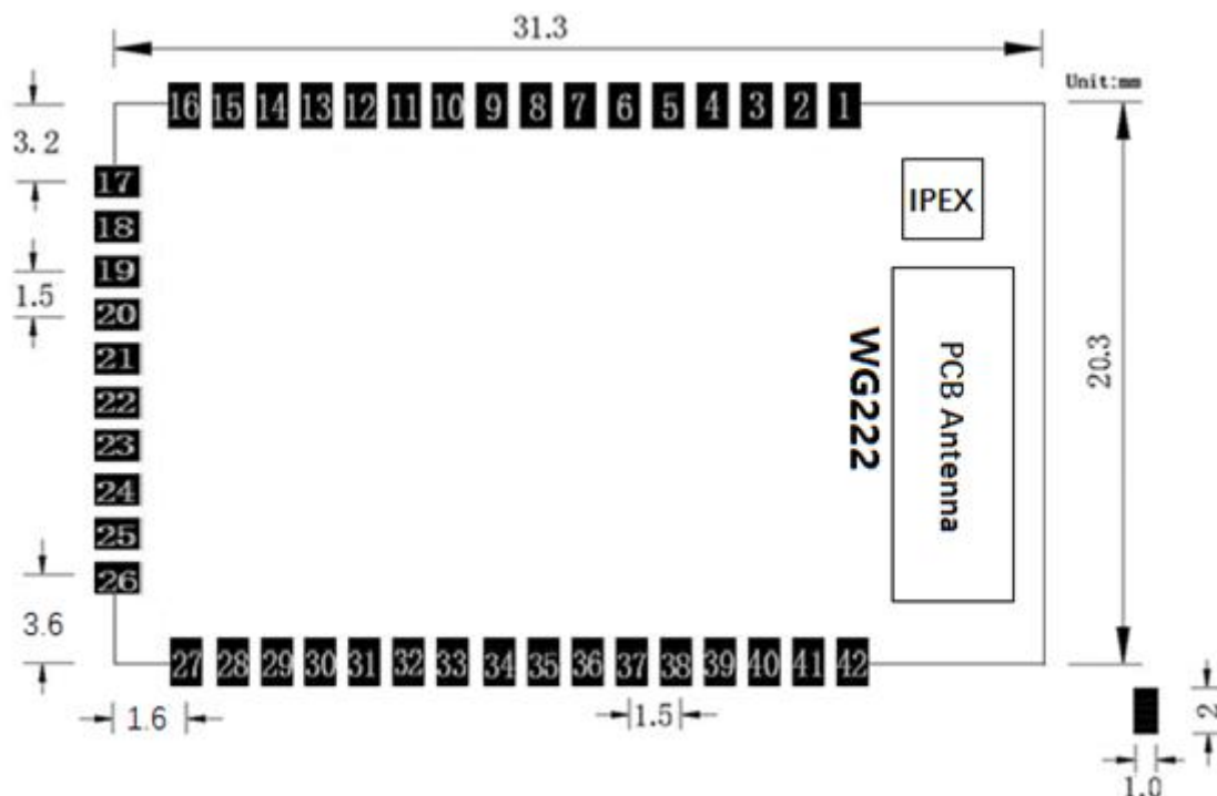
Figure 4: WG222 Dimensions
