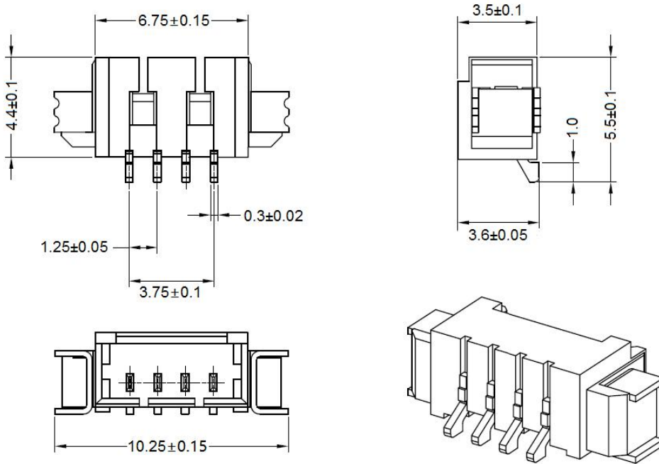
Figure 4: SKM80F Connector
