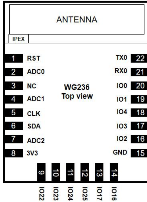
图 3: WG236 Pin封装/packaging
