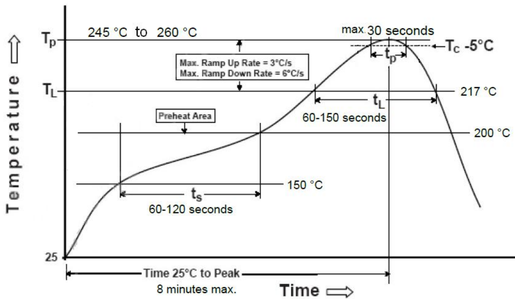
图 13-1 SKG122ER 推荐炉温曲线/ Figure 13-1 SKG122ER recommended furnace temperature curve
