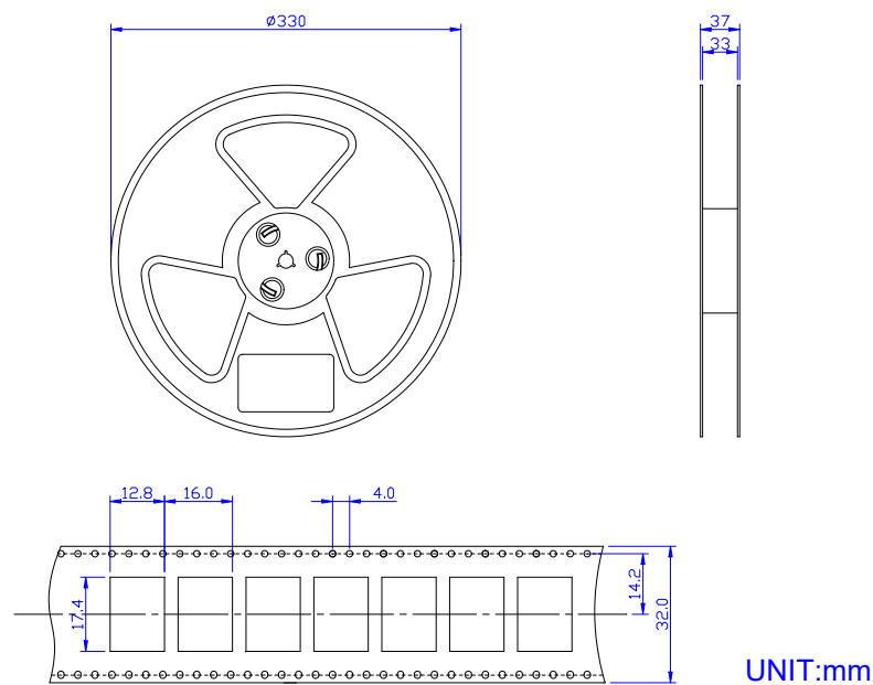
图 12-1 SKG122ER 包装图/ Figure 12-1 Packing diagram of the SKG122ER
