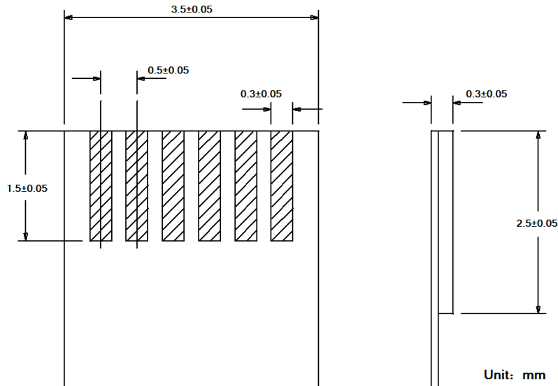
Figure 5: FPC/FFC cable
