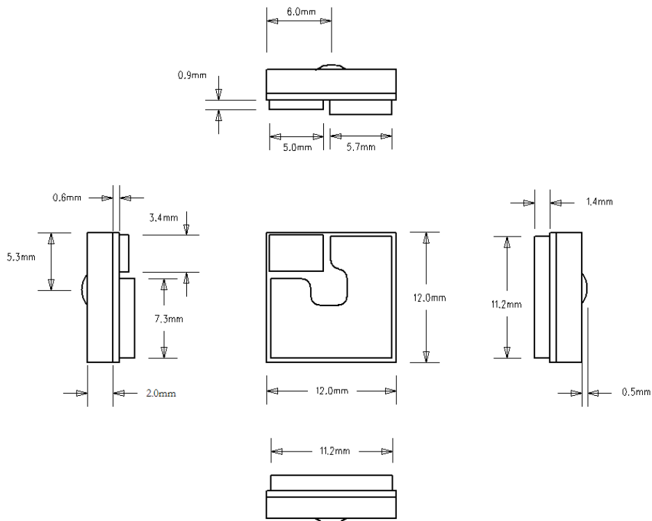
Figure 3: SKM56A-45 Dimensions
