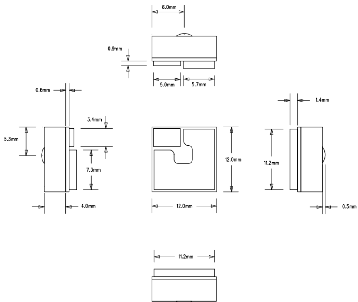
Figure 4: SKM56A-65 Dimensions
