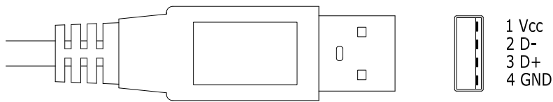
USB Connector
