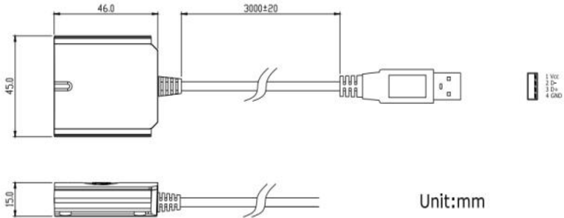
Figure 3: SKM55U-3GB Series Connector
