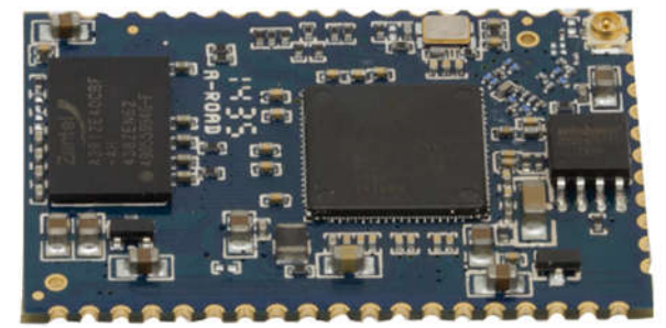
Figure 1: SKW72 Top View
