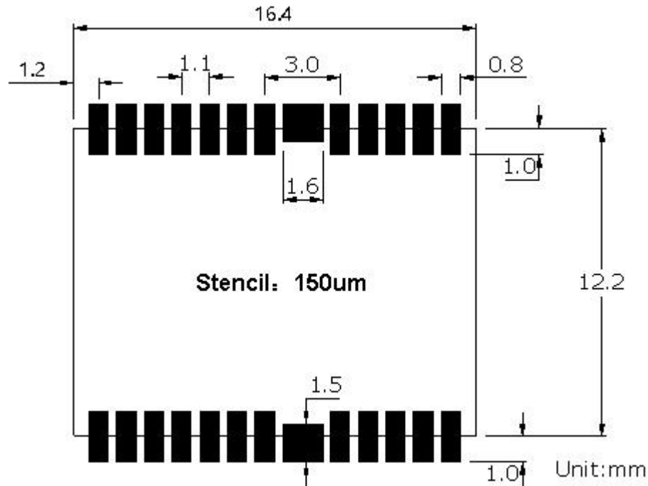
Figure 4: SKG12D Footprint
