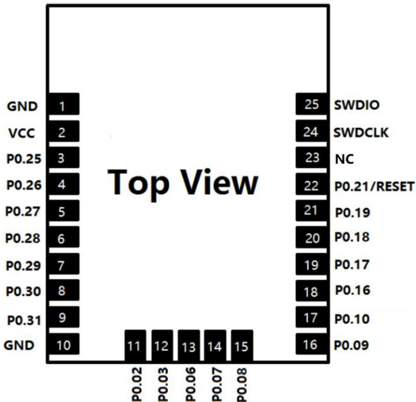
Figure 5: SKB376 Module Pinout
