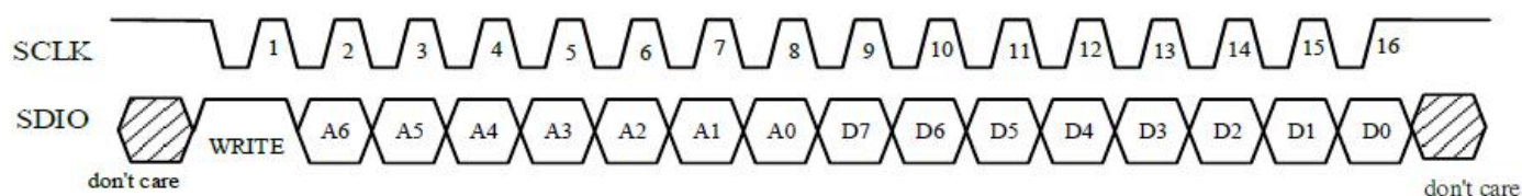
Figure 6-9 3-wire SPI write operation
