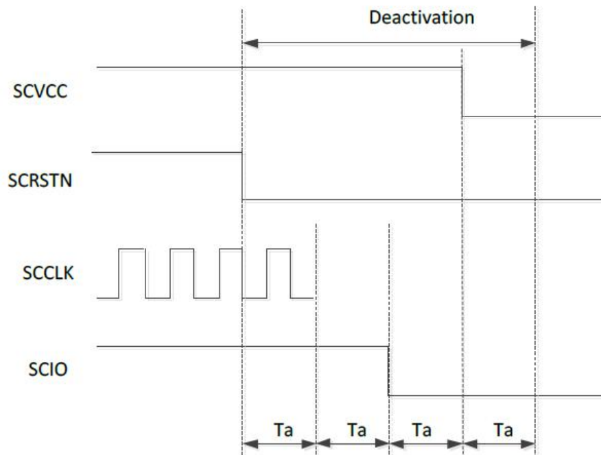
Figure 6-22 Deactivation Sequence
