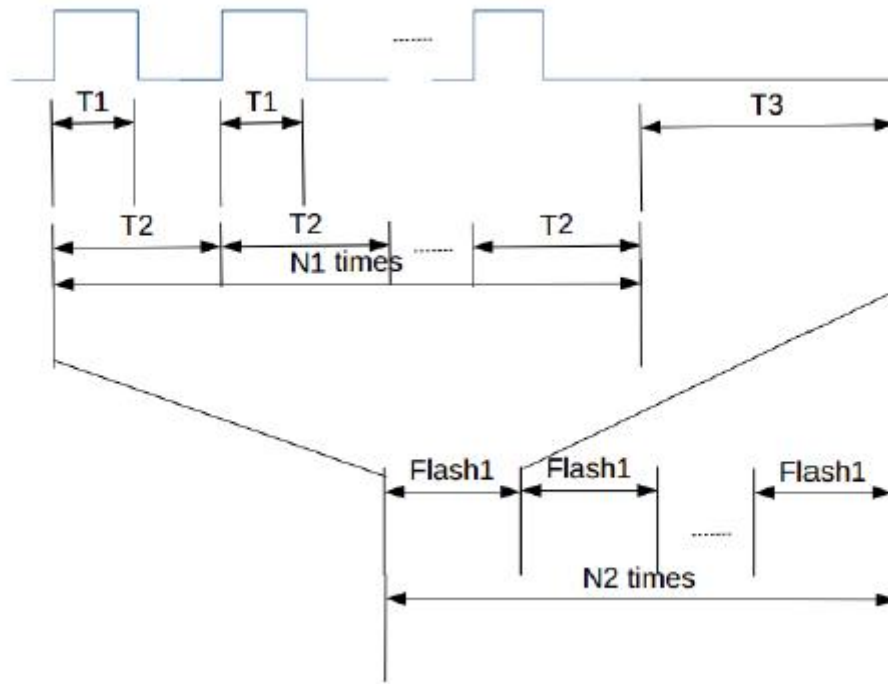
Figure6-18 LED on/off configuration
