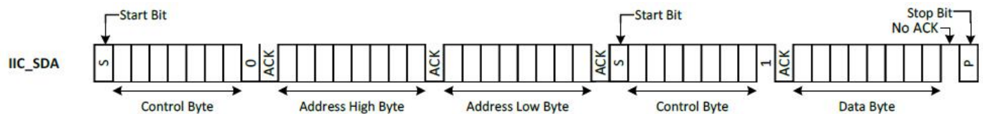
Figure 6-5 I2C random read format
