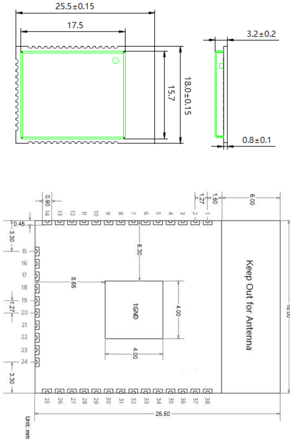
Recommend PCB Footprint
