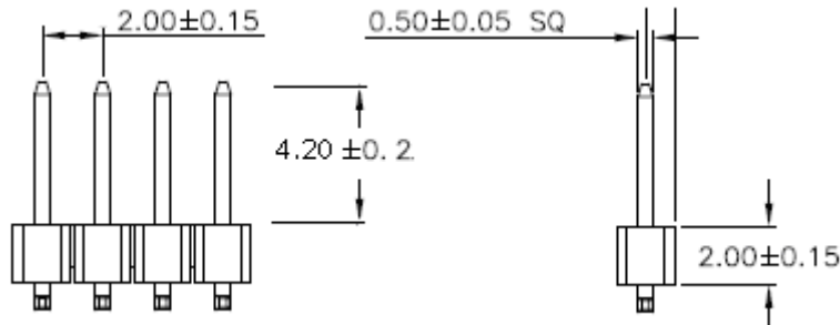
Figure 4: WG217 Dimensions
