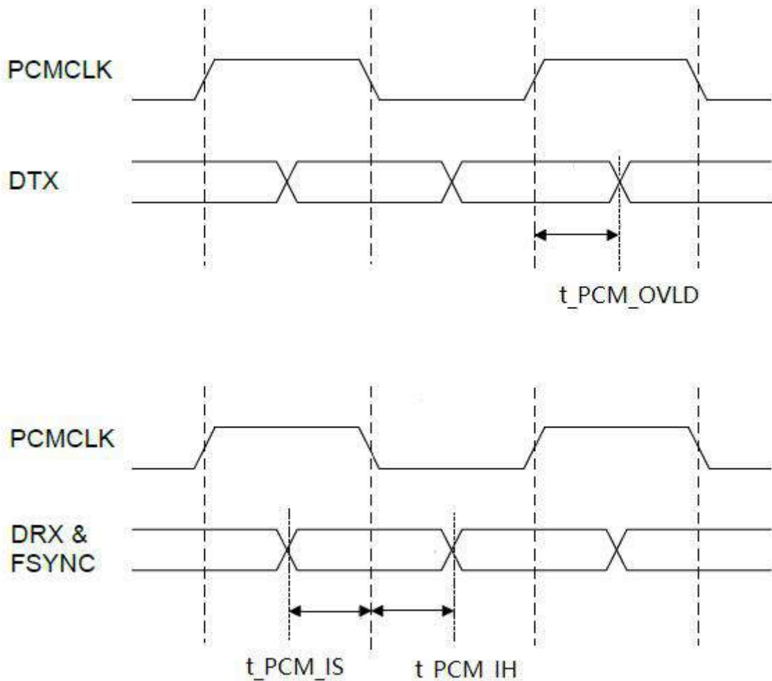
Figure 4: PCM Timing
